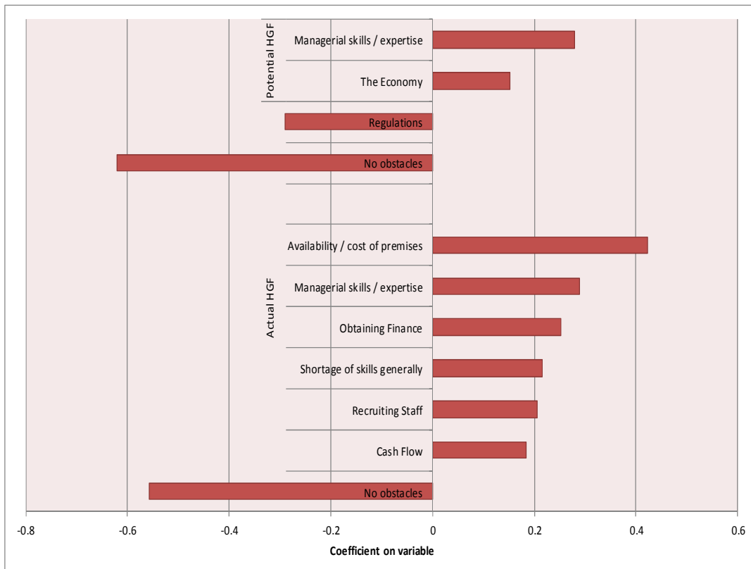
Figure 3: Regression coefficients
